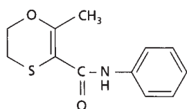
Carboxin (carboxamide)
