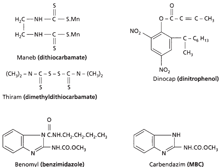
Fig. 17.3 Examples of protectant fungicides: maneb, thiram, and dinocap.
