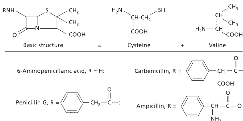
Fig. 7.16 Structure of penicillins.
